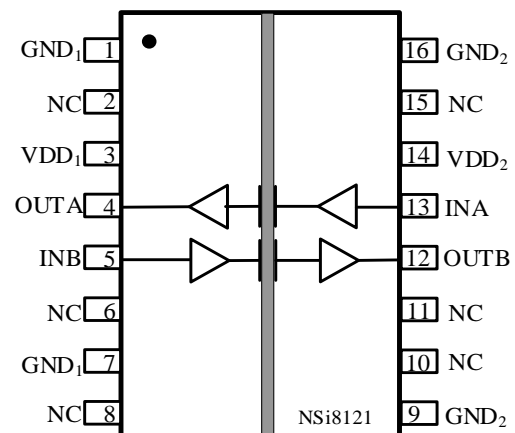
Figure 6.6 NSi8121W Package
