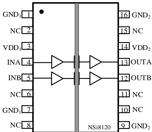
Figure 6.5 NSi8120W Package
