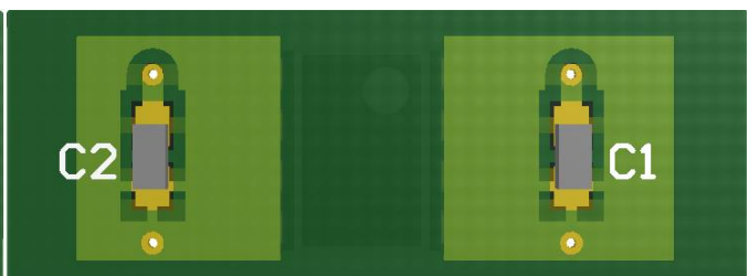
Figure 5.2 Recommended PCB Layout — Bottom Layer
